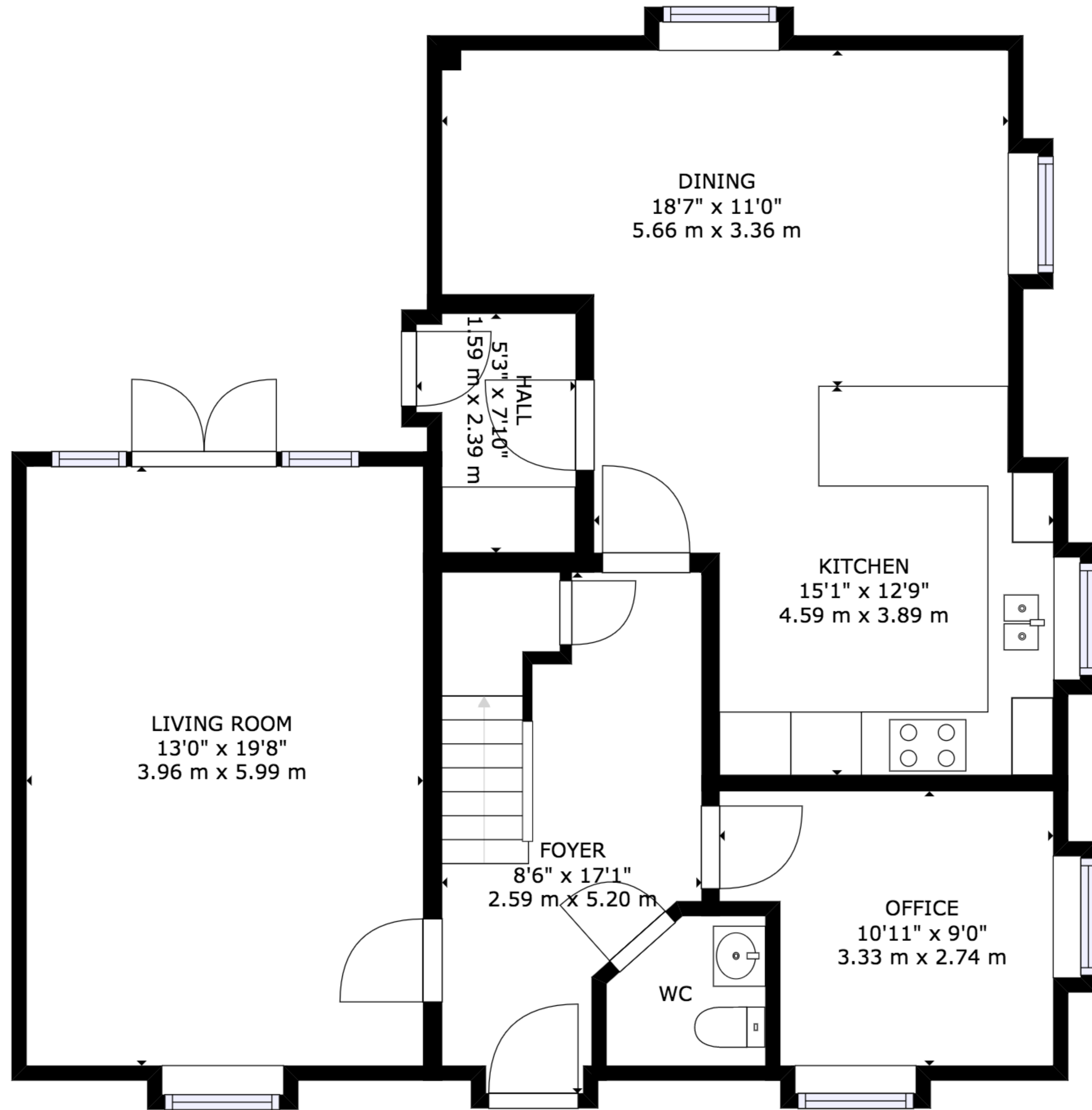
FLOOR 1
